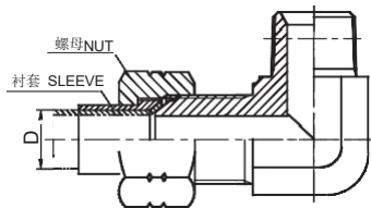
90° 弯 JIC外螺纹74° 外锥 / 布锥管外螺纹 90° ELBOW JIC MALE 74° CONE / NPT MALE
