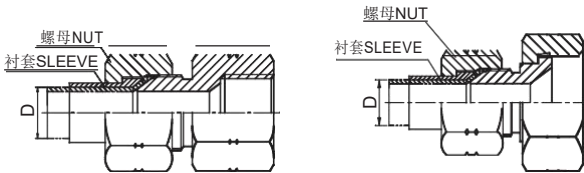
JIC外螺纹74° 外锥 / JIC内螺纹74° 内锥 JIC MALE 74° CONE / JIC FEMALE 74° SEAT
