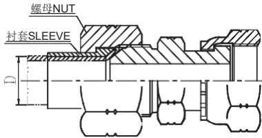
JIC外螺纹74° 内锥 / ORFS内螺纹 JIC MALE 74° CONE / ORFS FEMALE
