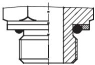
O形圈密封 O-Ring Seal
